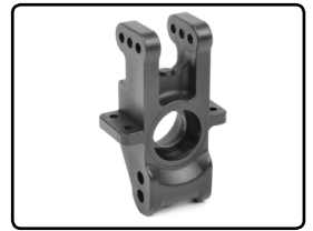
C-00180-008 Hub - Rear - Composite - 1 pc
